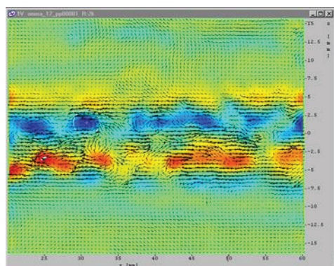
Figure 5 - Axial injection - PIV- Instantaneous velocity fluctuations (difference with mean values) and vortex strength
