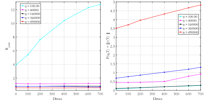
Fig. 2. Evolution of R_{\text{com}} , P(q, t) and \epsilon_0 for different values of D_{\text{max}} and \eta , with \eta_2 = 7.5 . The SS model (34) and the accurate estimator (16) are considered.
