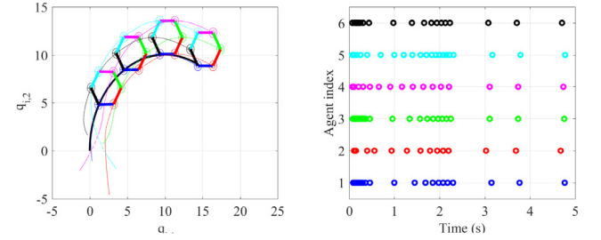
Fig. 3. Hexagonal formation and tracking problem with D_{\text{max}} = 20 , \eta = 50 , and \eta_2 = 7.5 . Circles represent agents (left figure) and communication events (right figure). R_{\text{com}} = 2.43\% , P(q, T) = 0.001 and \|\epsilon_0\| = 0.1 . T = 5 s.
