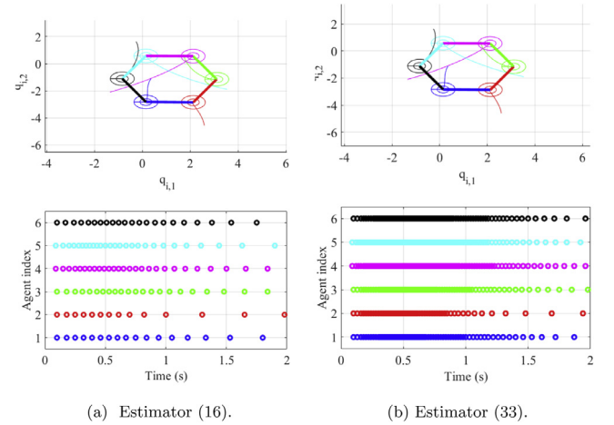
Fig. 4. Hexagonal formation with D_{\text{max}} = 20 , \eta = 20 and \eta_2 = 7.5 . Agents are represented by circles. In (a), R_{\text{com}} = 10.75\% and P(q, T) = 0.001 . In (b) R_{\text{com}} = 40.25\% and P(q, T) = 0.001 . T = 2 s.
