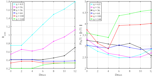
Fig. 1. Evolution of R_{\text{com}} and P(q, t) + \|\epsilon\| for different values of D_{\text{max}} and \eta , with \eta_2 = 7.5 . The DI model as well as the constant estimator (33) are considered.
